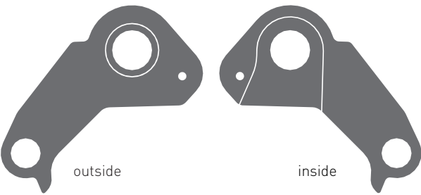
Hanger for SRAM & Shimano Standard
